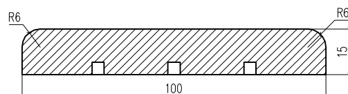
Listwa 100x15 R6
